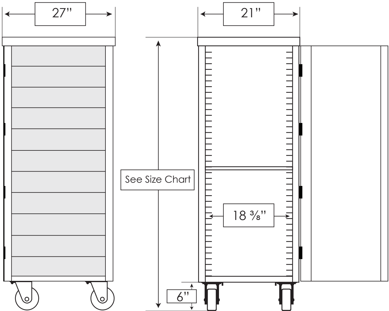
SIDE VIEW
